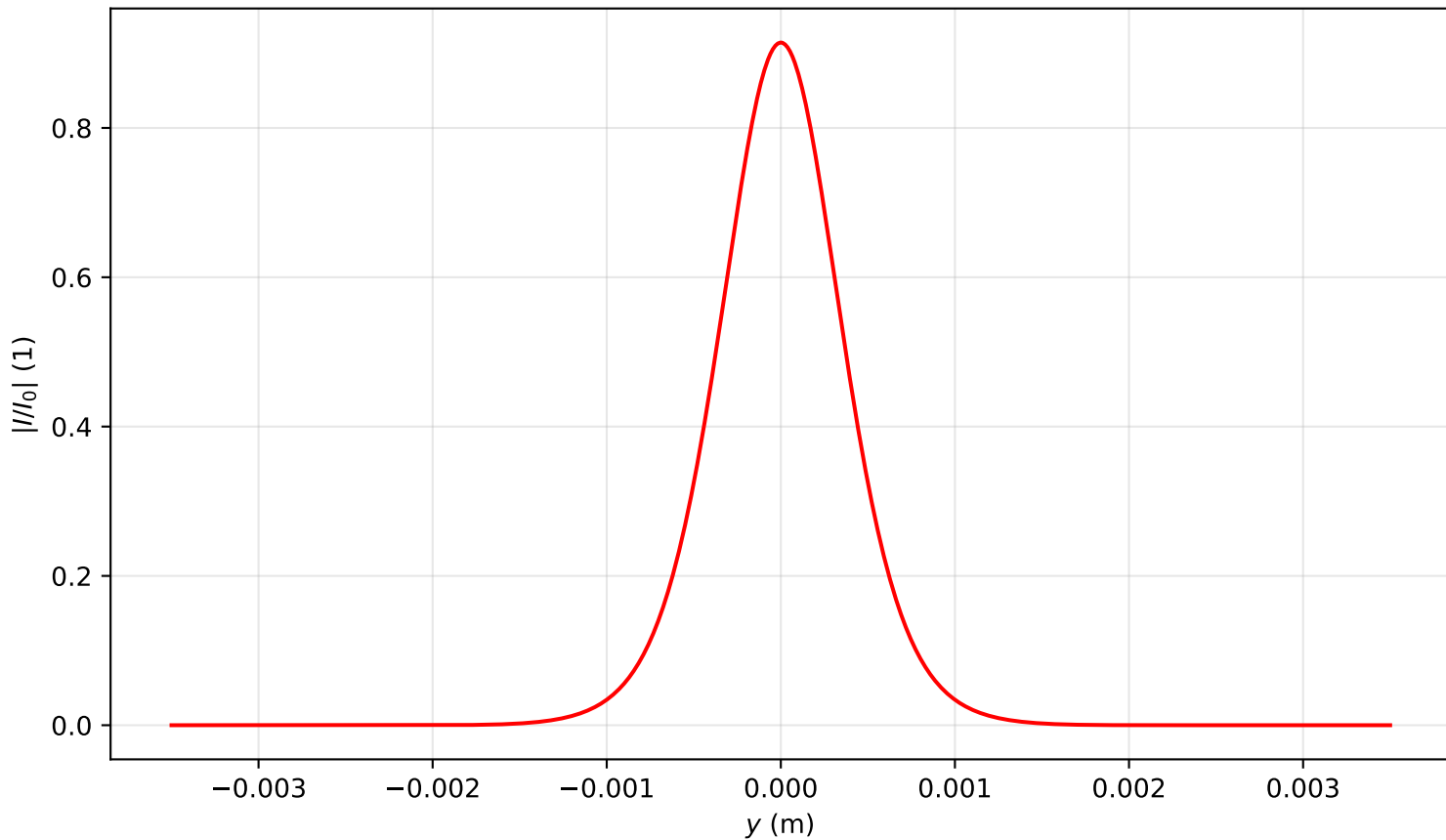
Intensity profile I(x=0, y, z=1.672)/I_0 , P_{in}=0.5P_{cr} , artificial time
